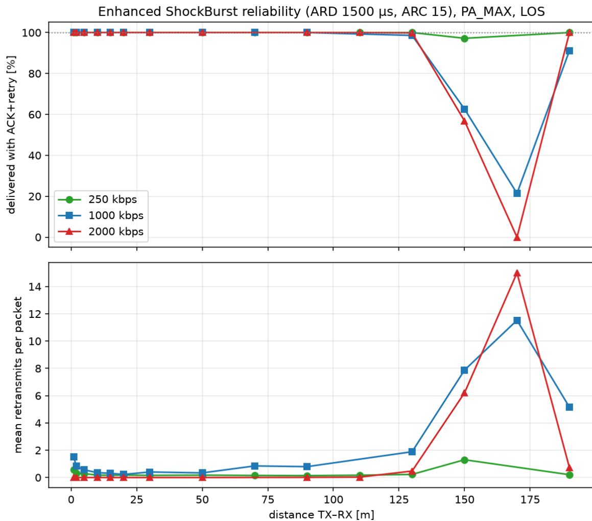
Figure 4: ACK Reliability vs distance
