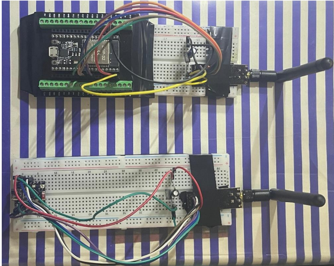
Figure 1: Physical hardware setup
