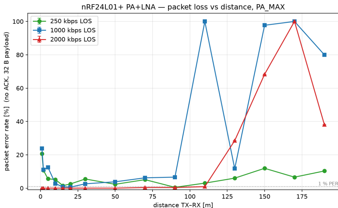
Figure 2: Packet-loss versus distance curves (LOS)
