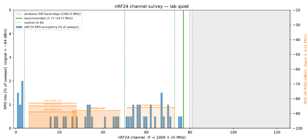
Figure 3: Channel survey spectrum analysis and Wi-Fi AP interference overlay
